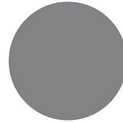
Dalton
