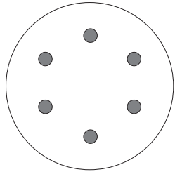
Thomson
